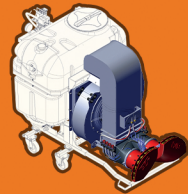
D52 (Orchard) - Up to 6 mtrs Interrow distance D52Ø - 55 Hp - 185 Kgs
